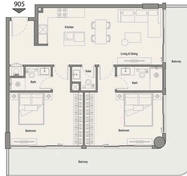
UNIT 905 - 2 BEDROOM
